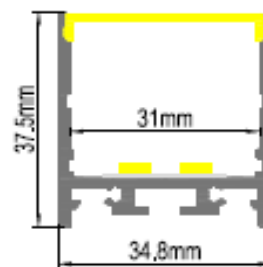
BR-S-ALP-024x Powerline profile -PMMA Diffuser
