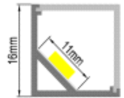
BR-S-ALP-022x Corner Profile -PMMA Diffuser
