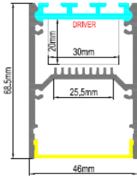
BR-S-ALP-026x Driver Profile - PMMA Diffuser
