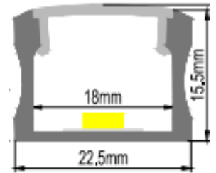
BR-S-ALP-029x Surface Mounted profile -PC Diffuser
