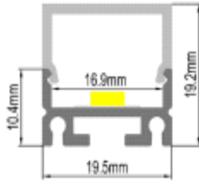
BR-S-ALP-039x Ceiling Profile -PMMA Diffuser
