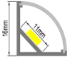
BR-S-ALP-014x Corner Profile - PMMA Diffuser
