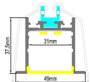
BR-S-ALP-025x Powerline profile -PMMA Diffuser
