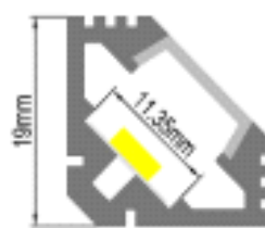
BR-S-ALP-037x Corner Profile -PC Diffuser
