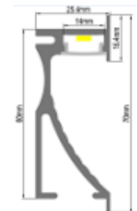
BR-S-ALP-050x Wall Profile -PMMA Diffuser
